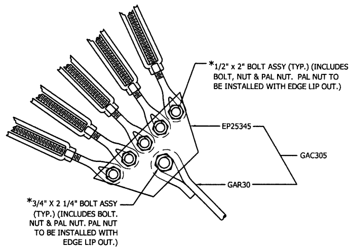
FIVE WIRE ATTACHMENT
