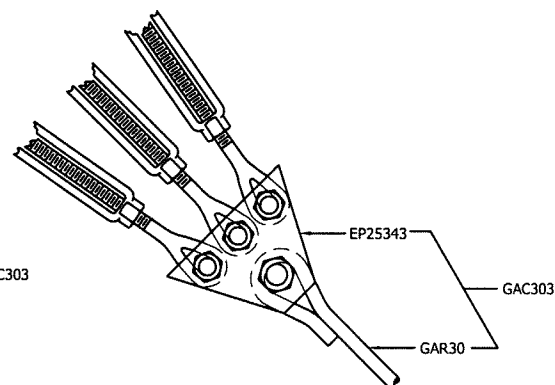
THREE WIRE ATTACHMENT
